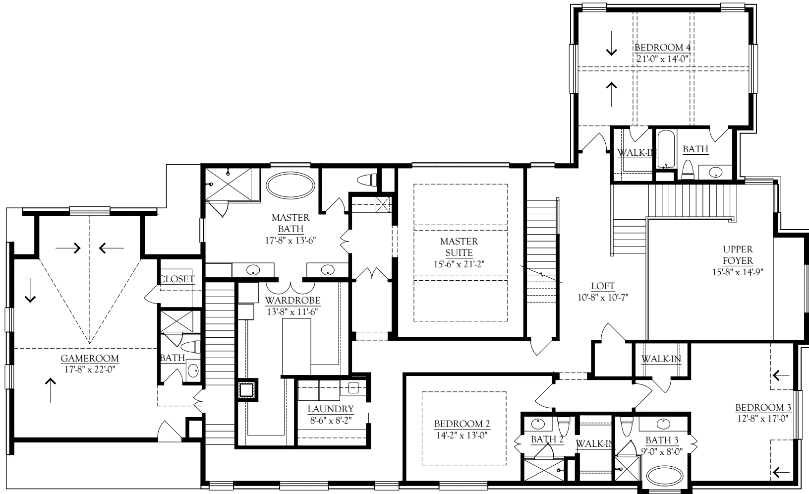
SECOND LEVEL FLOOR PLAN
