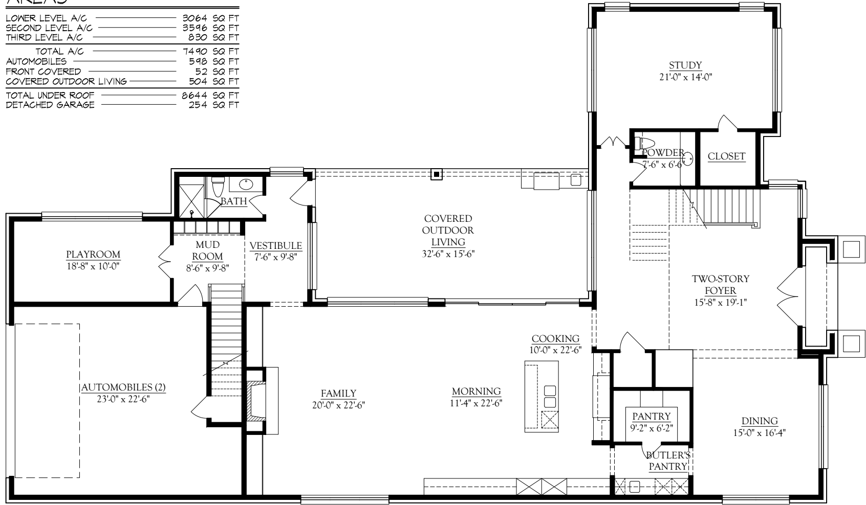
LOWER LEVEL FLOOR PLAN
